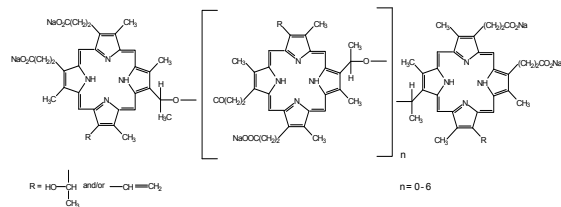
Figure 1 Structure of Porfimer Sodium
